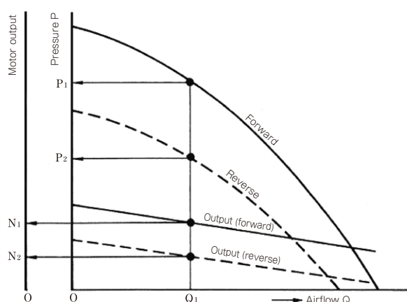
Characteristics with reverse operation
