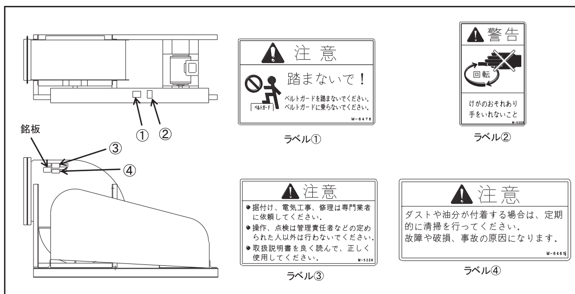
図1 警告ラベル配置例(CLF II (R)-No.3-TH-L-RS)
